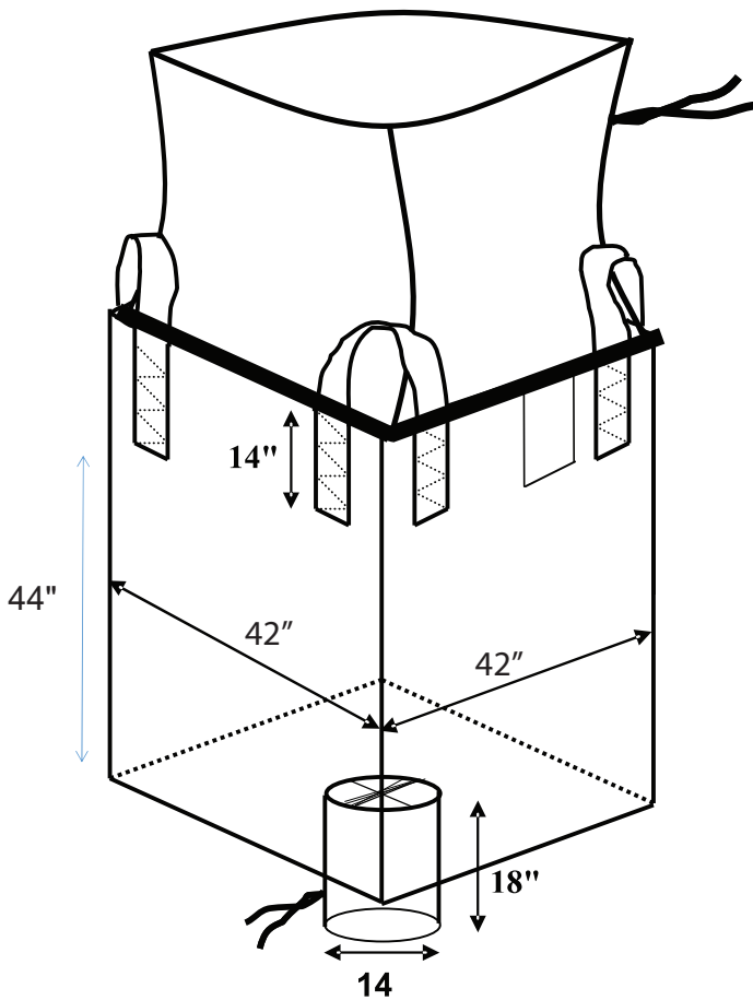
DRAWING FOR 42X42X44 CROSS CORNER , D/S, 3000 LBS (BAFFLES)
